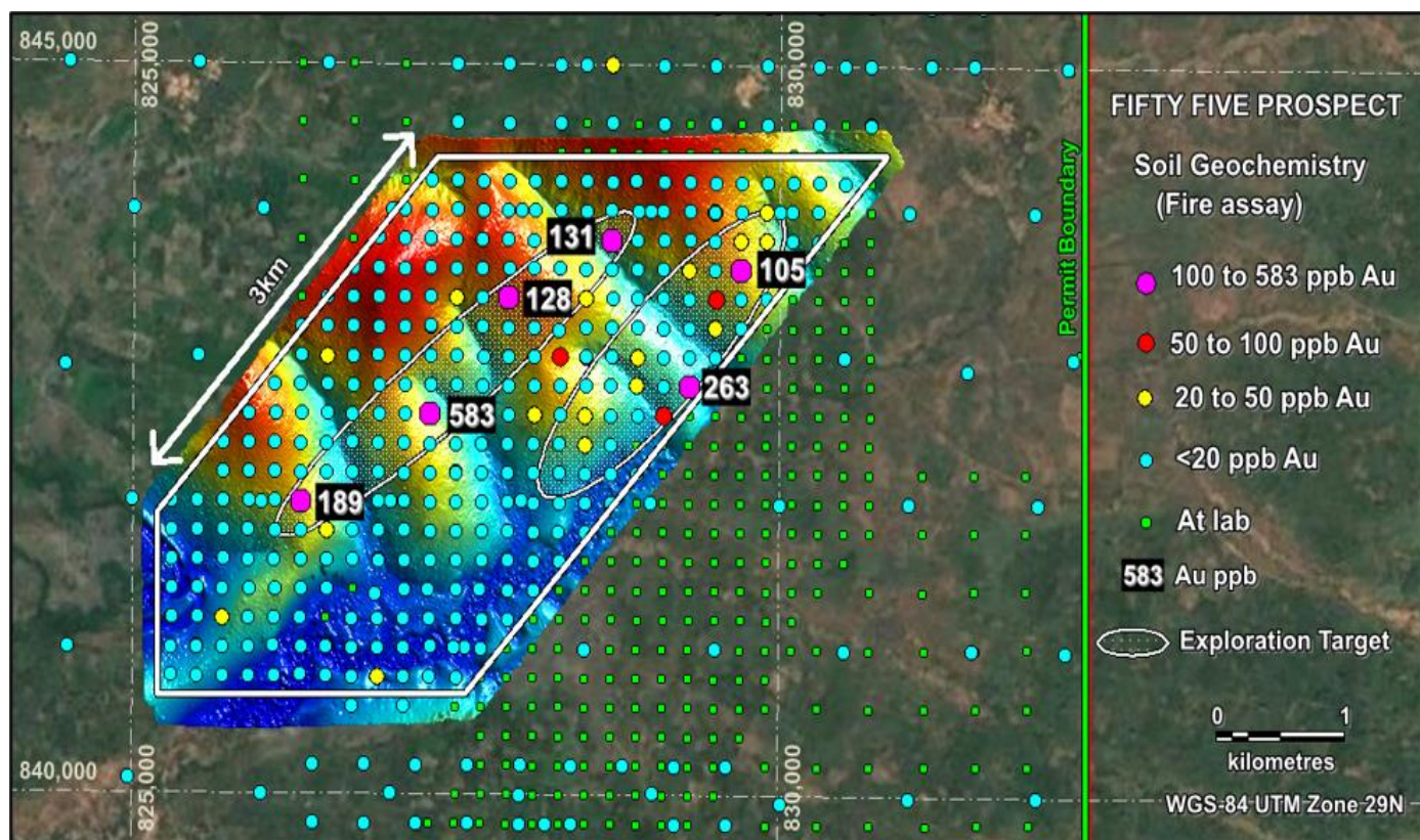
Figure 1. Zuénoula soil sampling progress on LiDAR topographical image Red and Orange: high ground. Blue: low ground with transported soil cover
