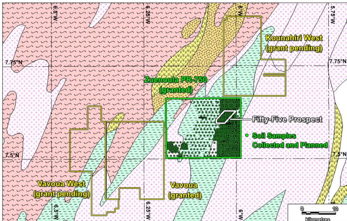
Figure 2. Location of Zuénoula permit and the Fifty-Five Prospect within Zuénoula
